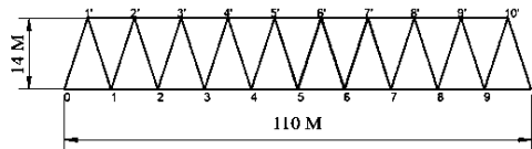
Figure 3: The superstructure of a metal bridge (truss).
