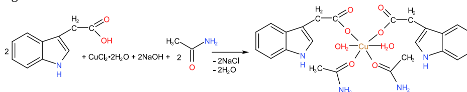
1-rasm. [\text{Cu}(\text{IAA})_2(\text{AA})_2(\text{H}_2\text{O})_2] kompleks birikmasining sintez reaksiyasi
