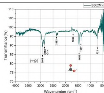
2-rasm. SM BEU -2 namunasining IQ-spektri.
