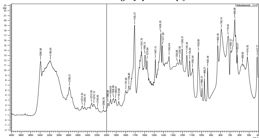
4-rasm. [\text{Cu}(\text{IAA})_2(\text{AA})_2(\text{H}_2\text{O})_2] kompleks birikmasining IQ-spektroskopiya tasviri
