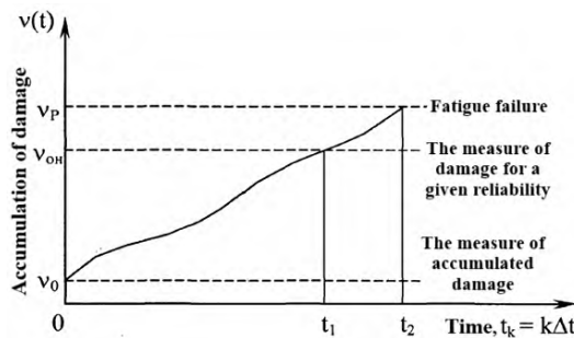
Figure 1: The scheme of accumulation of damage in the element
