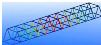
Figure 5: The result of the work: color display of the degree of accumulated damage in the bridge elements.
