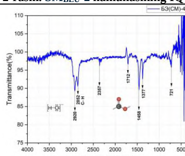
4-rasm. SM BEU -4 namunasining IQ-spektri.
