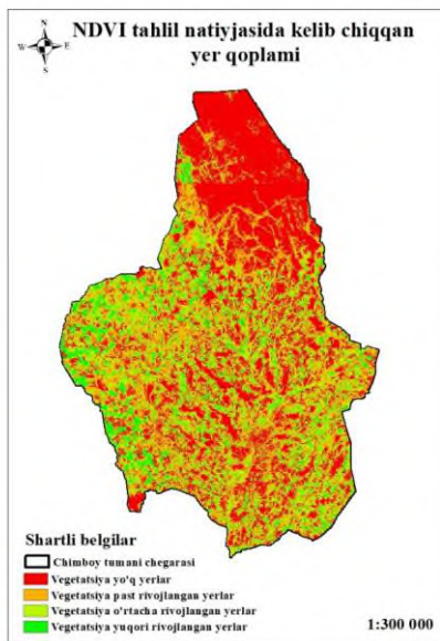
4a-rasm. Chimboy tumanining yashillik bilan qoplanish darajasi 2018 yil holatiga
