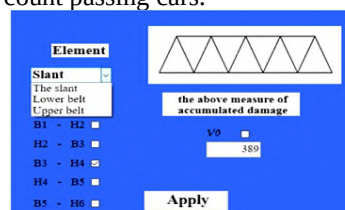
Figure 4: The dialog box of the element reliability assessment program.
