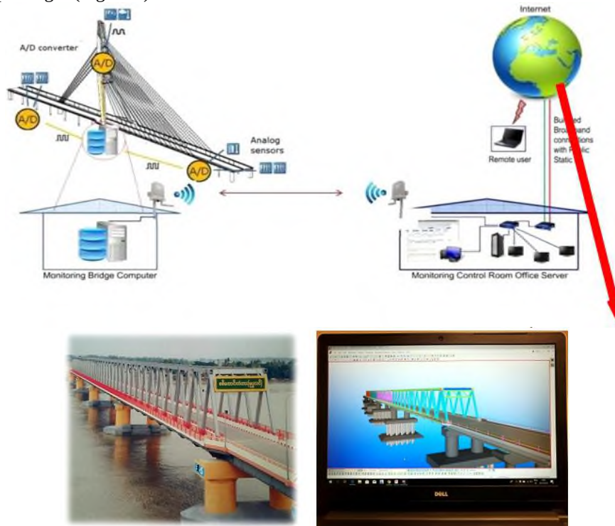
Figure 2: Transfer of monitoring results to the information model
